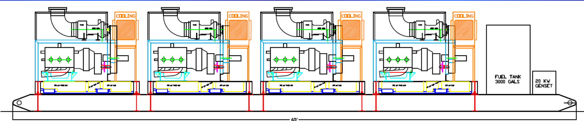
65 Foot Quad Frac Skid Designed for Semi-Permanent Walking Rigs. All Frac Units Run on #2 Diesel, CNG, LNG, Field Gas & Bio-Fuel
