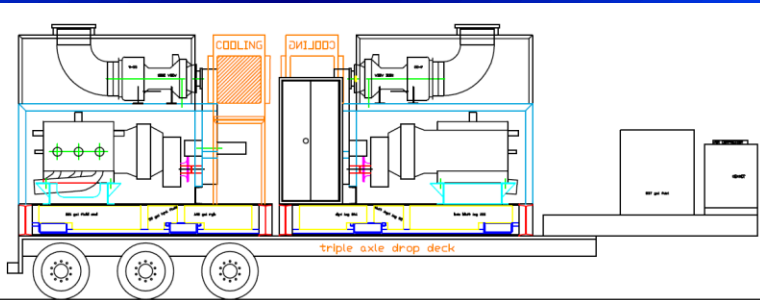
35 Foot Double Frac with Fuel Storage and 25 KW Gen
