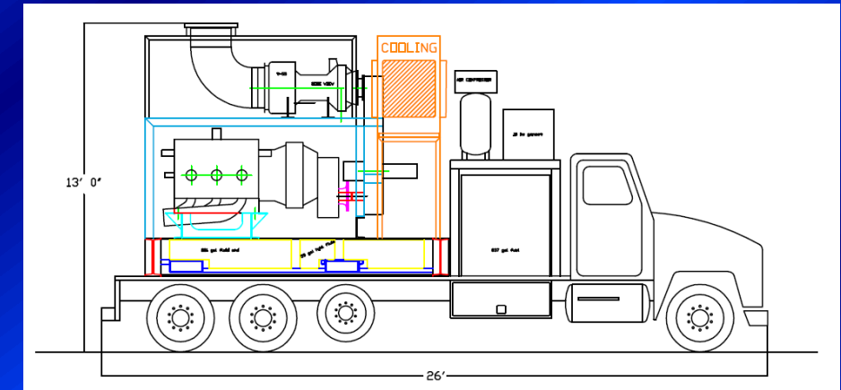
Bobtail Frac for Marcellus Shale and Tight Access Sites. 26 Foot Frac Unit
