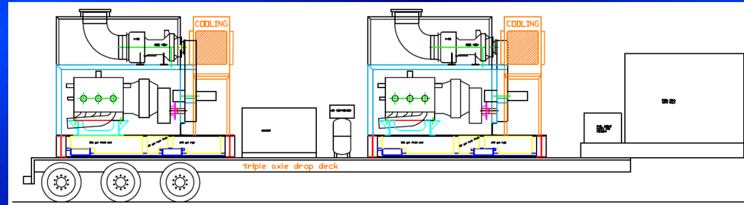
48 Foot Double Frac with 3,000+ Gal Fuel, 25 KW Gen and Frac Support Accessories
