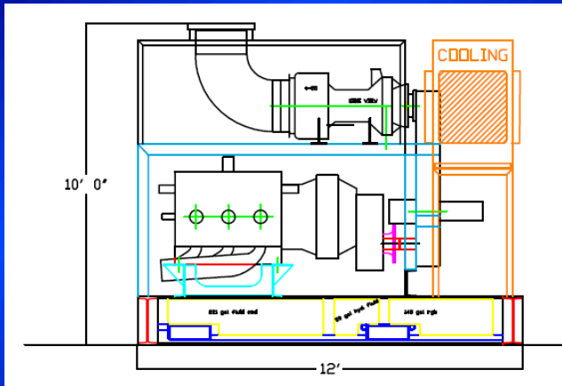
Plug & Play Spare. Offshore Transport - 23,000 lbs
