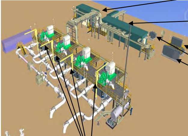
TYPICAL PUMP STATION LAYOUT
